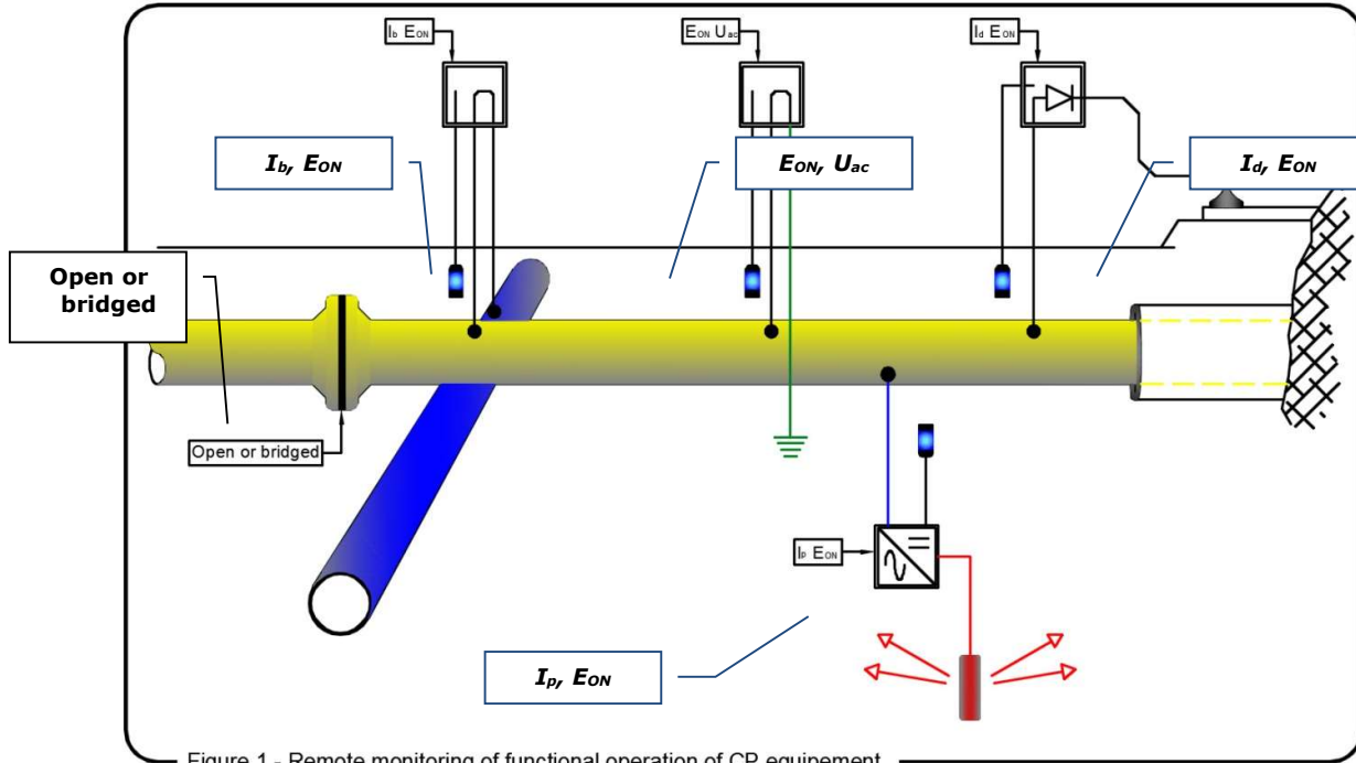
Figure 1 - Remote monitoring of functional operation of CP equipment
