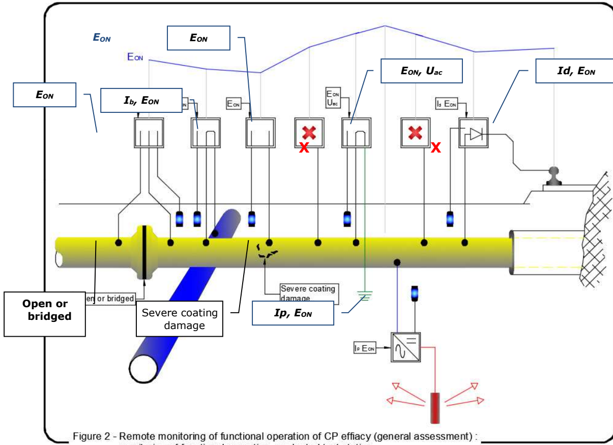
Figure 2 – Remote monitoring of CP efficacy (general assessment): monitoring of functional operation + selected test stations
