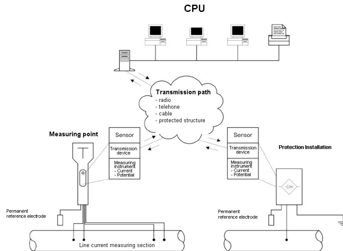
Figure 1 – General scheme of remote monitoring CP system
