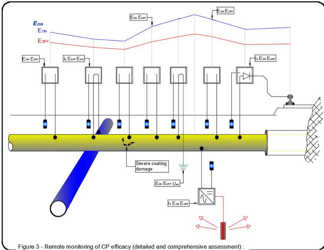
Figure 3 - Remote monitoring of CP efficacy (detailed and comprehensive assessment) : monitoring of functional operation + all test stations
