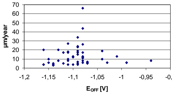
Figure 21: Uniform corrosion related to E OFF .
