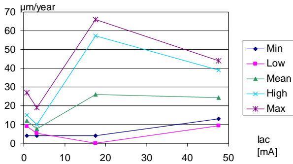
Figure 15: Uniform corrosion related to I_{ac} .
